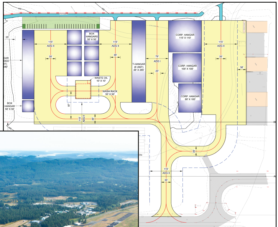
*Conceptual drawing
